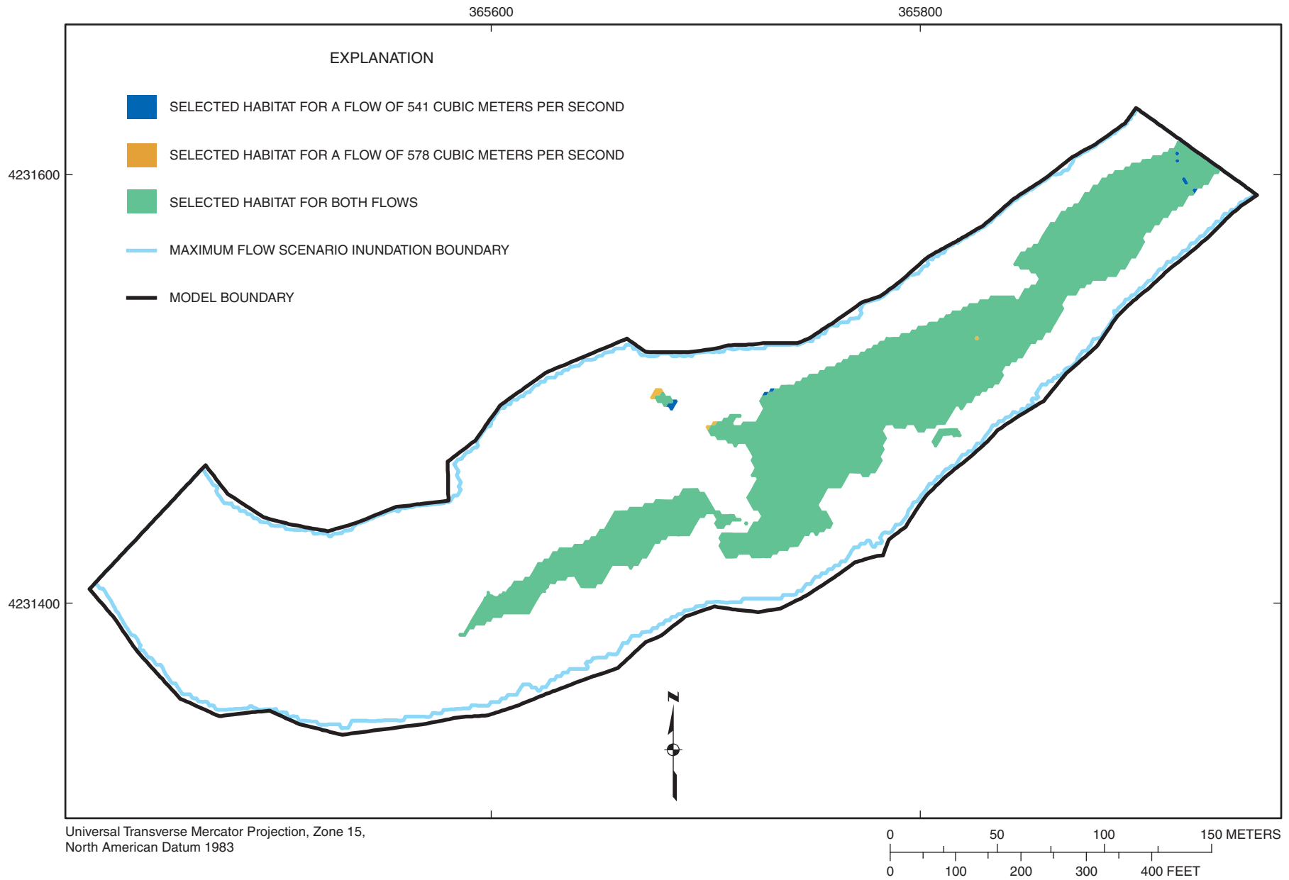
Figure 4-42. Selected habitat area distribution for habitat category 7 (paddlefish) at flows of 541 and 578 cubic meters per second at Marais des Cygnes River site MDC2.
